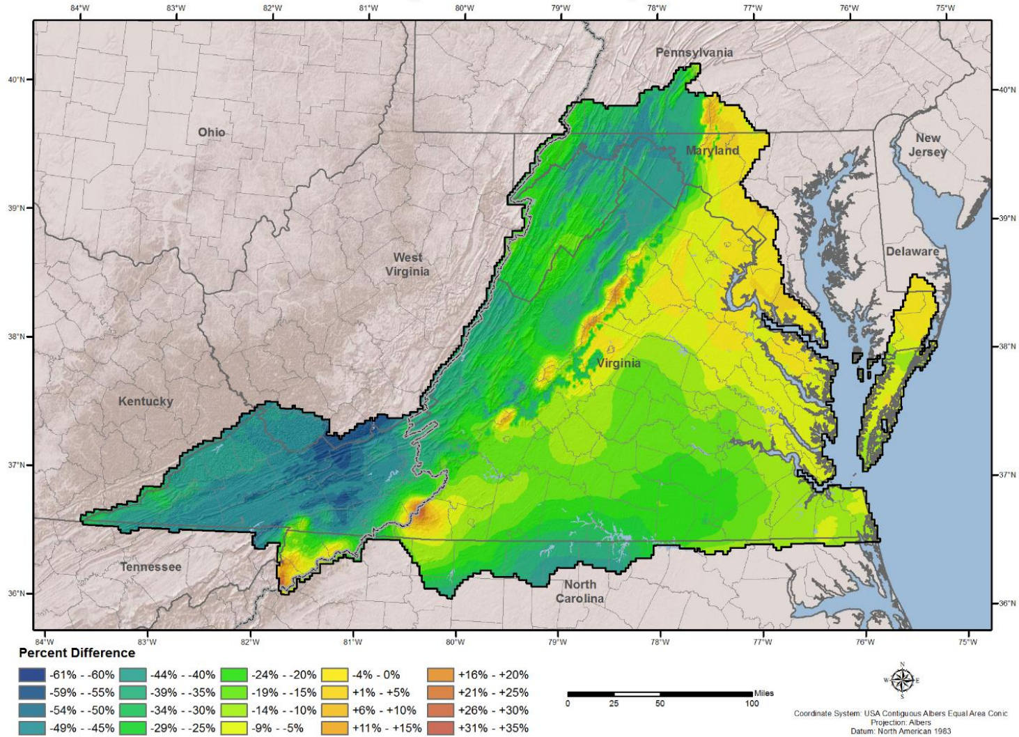
Figure 10.16 Percent difference of HMR 51 values compared to largest PMP values from all three storm types 72-hour 1,000 square miles. Note the scale in the legend is specific to the image.
